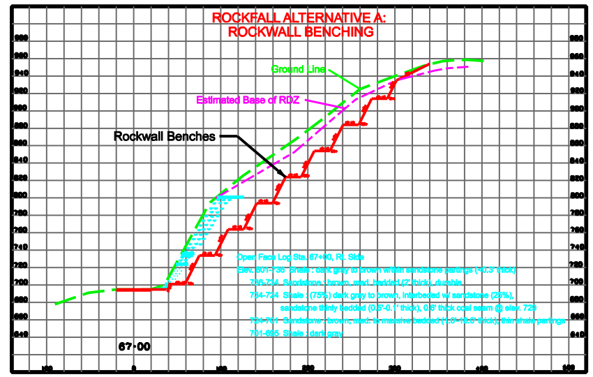
Rockfall Benching
